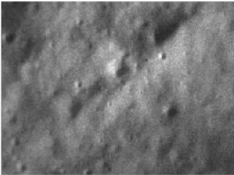
Fig. 1. The ruin-like formation near the lunar crater Lovelace photographed by the space probe Clementine on March 8, 1994 (image LHD 30055.080). This cluster of rectangular depressions occupied an area of about 13km 2 .
