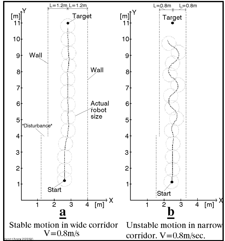
Figure 6: Motion in narrow corridors with f_{av}=0.8 , n=2 , T=0.065\text{sec} , \tau=0.3\text{sec} , V=0.8\text{m/sec} . a. Motion is stable if the corridor is sufficiently wide. b. Unstable motion in a narrow corridor.
