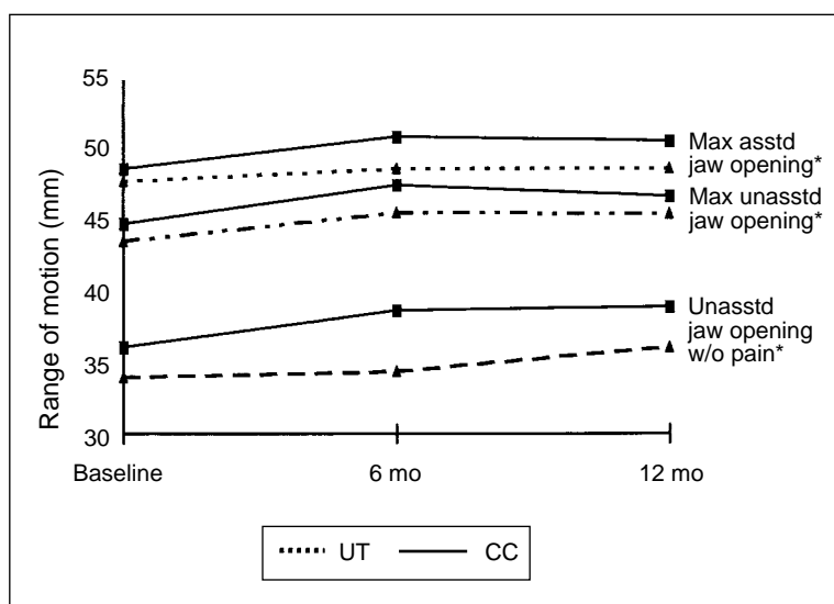
Fig 4 Comprehensive care versus usual treatment: Comparison of vertical range of jaw motion (in mm) for unassisted jaw opening, no pain; maximum unassisted jaw opening; and maximum assisted jaw opening. *All P values > .15 (ANOVA comparing groups at post-treatment and 1-year follow-up).
